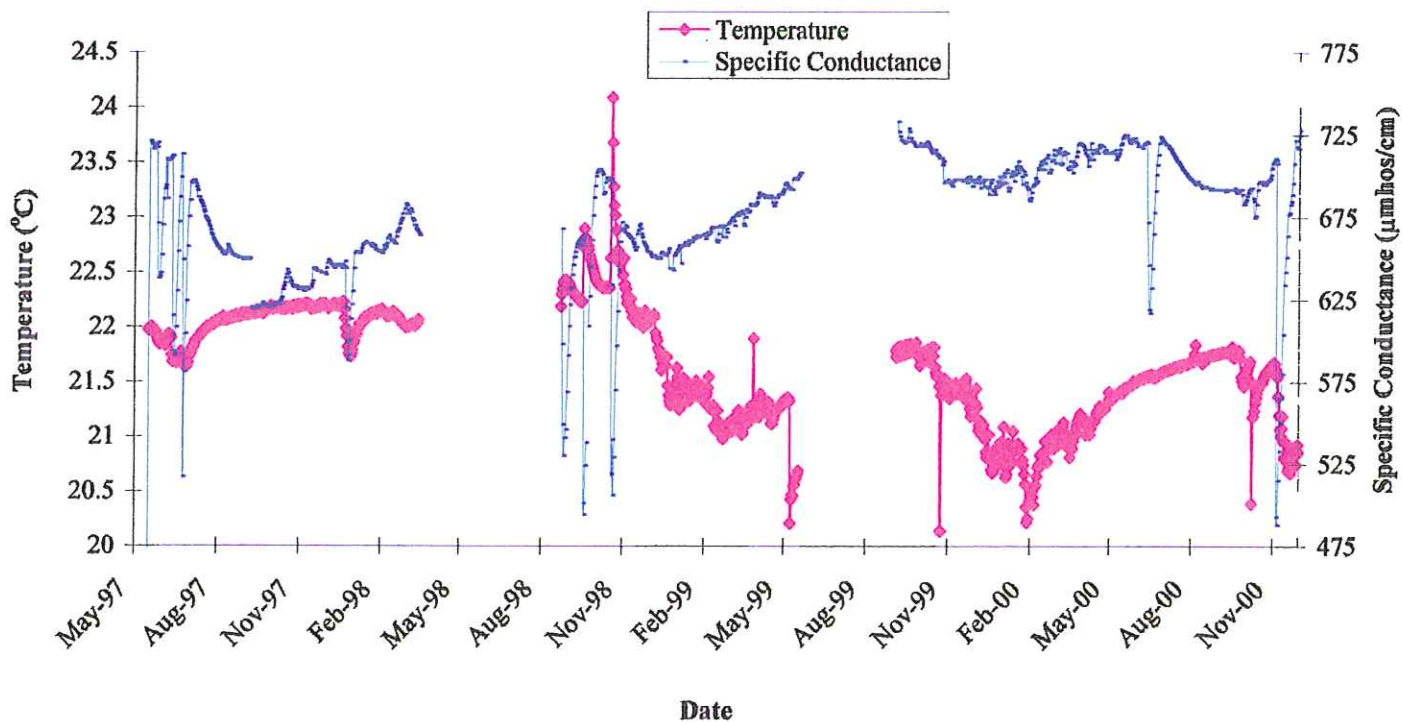
Fig. 8. Temperature (°C) and Specific Conductance (µmhos/cm) at Ezell's Cave Lake, 1997-2000
