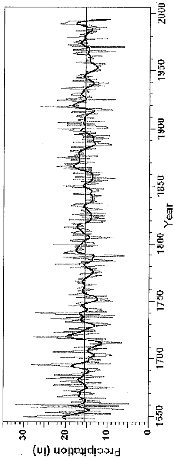
Figure 4. Reconstructed S. Central climatic division Feb. – June precipitation.
