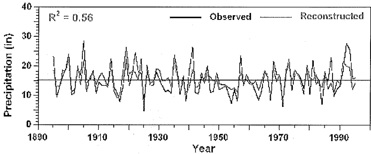
Figure 2. Calibration of Texas climate division South Central with a composite post oak chronology.
