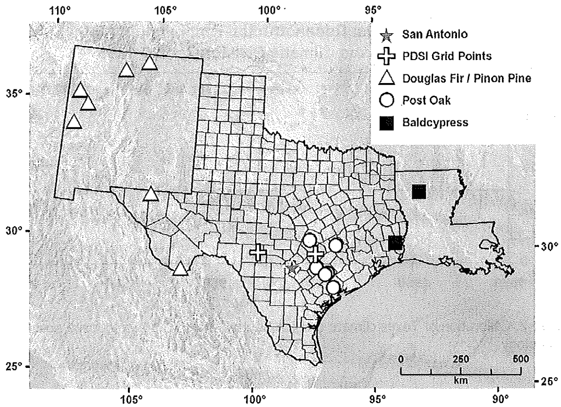
Figure 1. Map of area of reconstructions. Heavy black lines within the boundaries of Texas outline climate division 7 (S. Central) mainly to the east of San Antonio and climate division 6 (Edwards Plateau) mainly to the west of San Antonio. San Antonio lies within division 7 near its western border.
