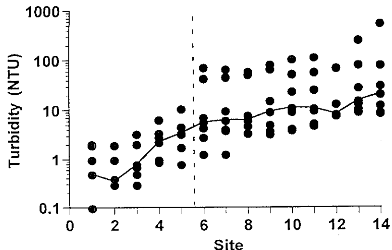
Figure 4. Turbidity on seven dates at sites along the San Marcos River. The solid line is the median. The vertical dotted line is the confluence with the Blanco River.
