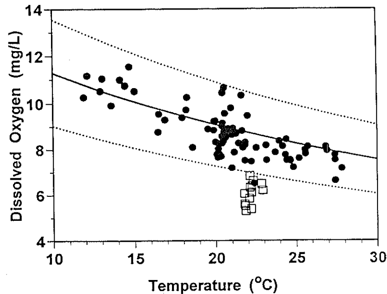
Figure 3. Relationship between dissolved oxygen and temperature in the San Marcos River at 14 sites. The solid and dotted curves represent 100% ( \pm 20\% ) oxygen saturation concentration at an atmospheric pressure of 760 mm Hg at sea level. The unfilled squares represent sites 1 and 2, the artesian well and Spring Lake, respectively. The filled symbols represent the other 12 sites.
