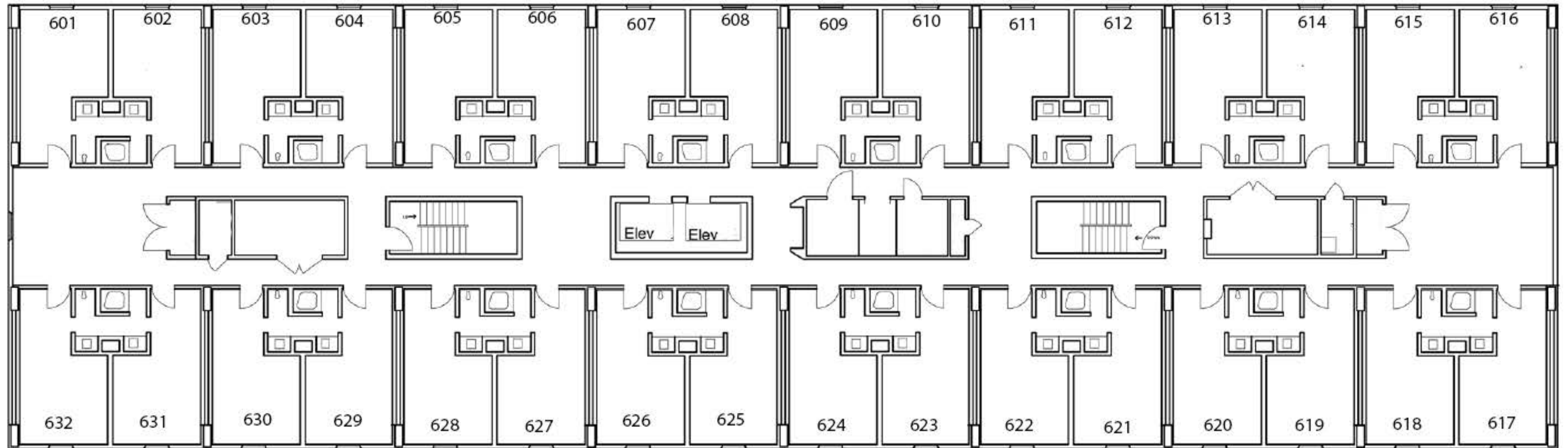
Tower Hall-Floor 6
