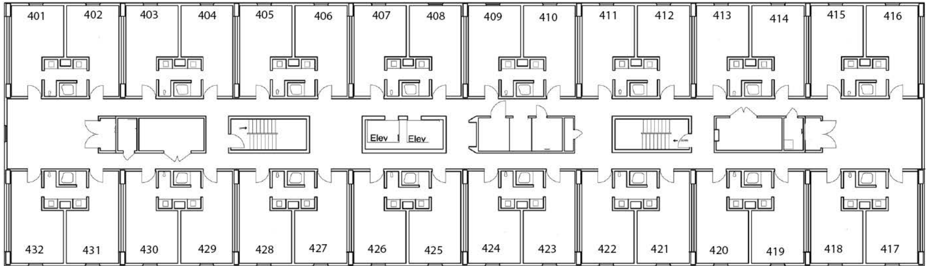
Tower Hall-Floor 4
