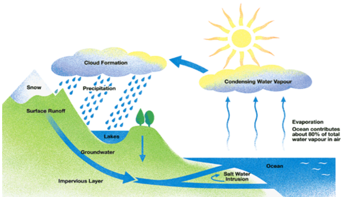
Diagram 1: Cycle of Evaporation, Precipitation, Recharge, and Runoff 5
