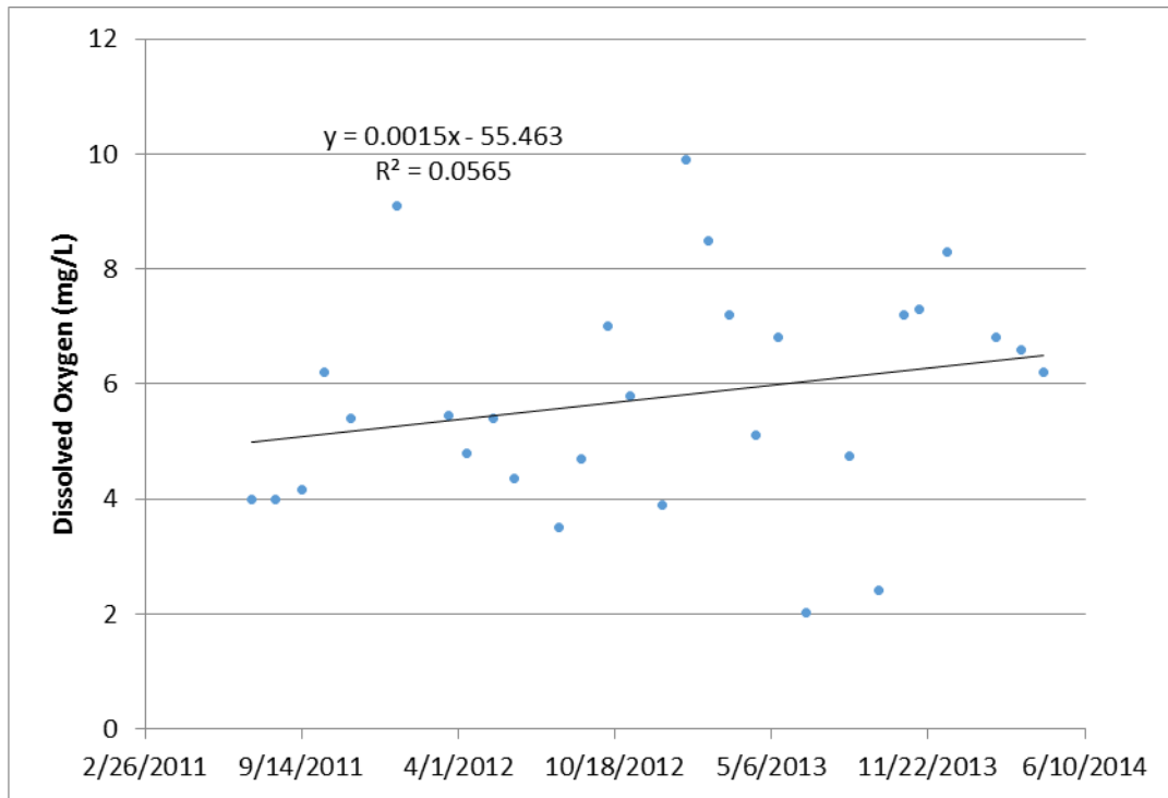
Figure 15: Dissolved Oxygen at Site 80680
