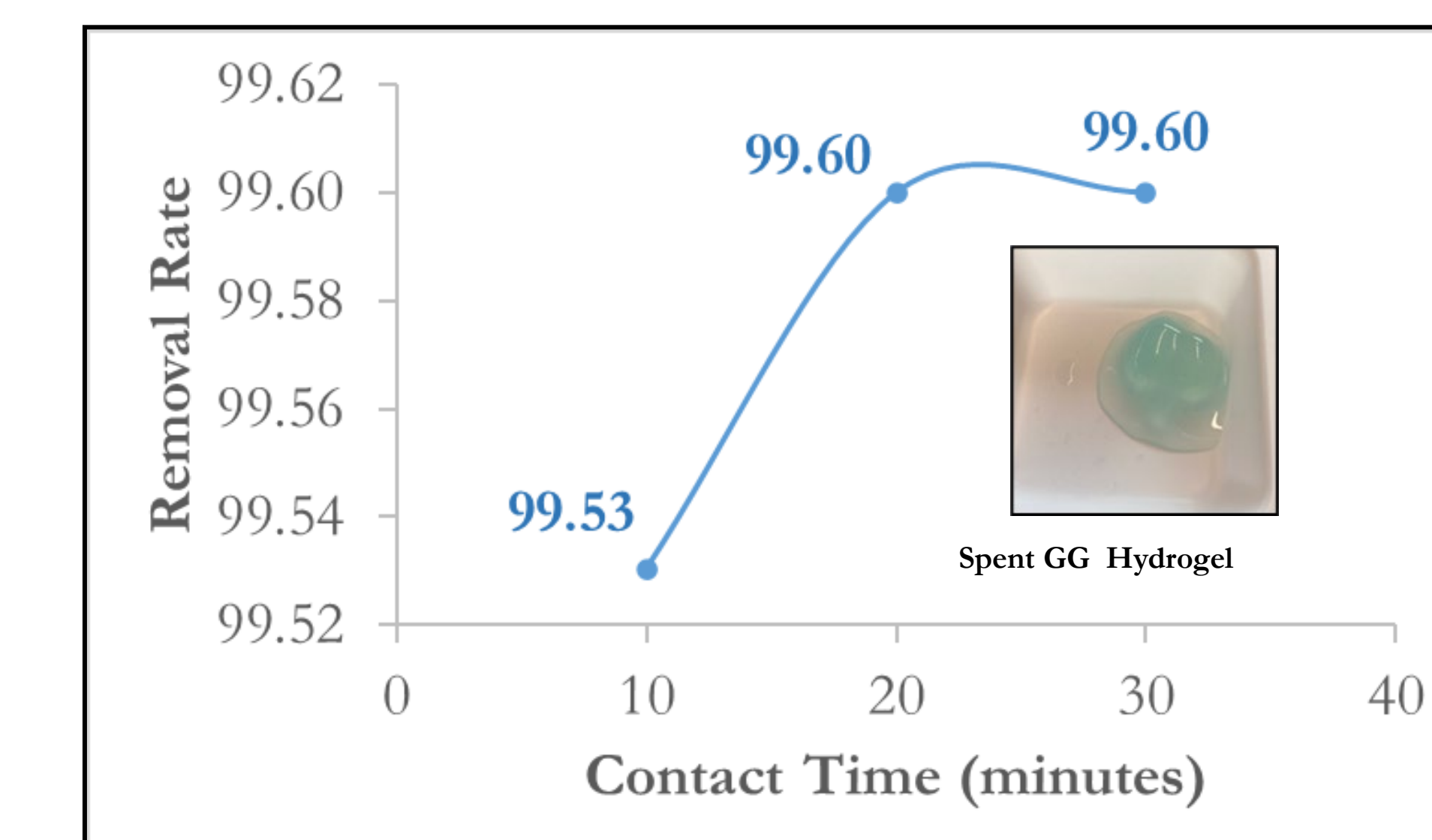
Removal Rate of MG dye from wastewater using GG hydrogel at three different contact time
