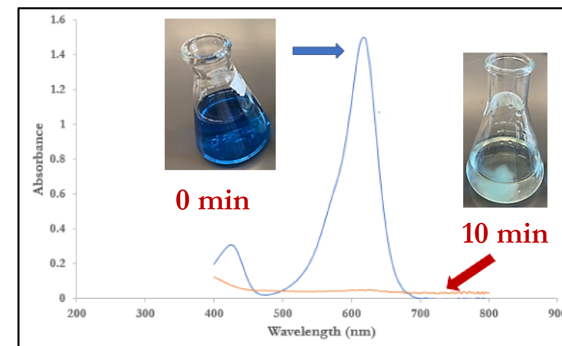
UV-VIS spectra of MG dye before and after adsorption by GG hydrogel at different time
