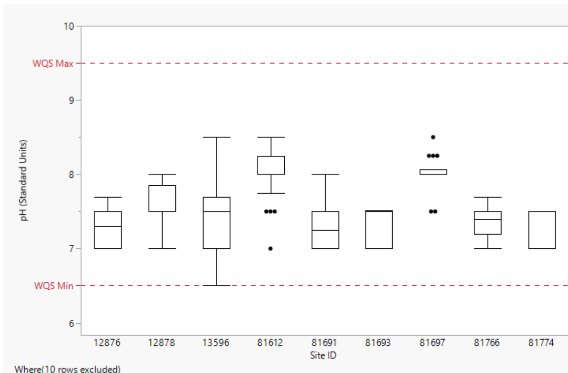
Figure 9. pH for Texas Stream Team sites in the Headwaters of Salado Creek watershed in Bexar County, Texas (November 1992 to January 2025). WQS Max = Maximum Water Quality Standard; WQS Min = Minimum Water Quality Standard.
