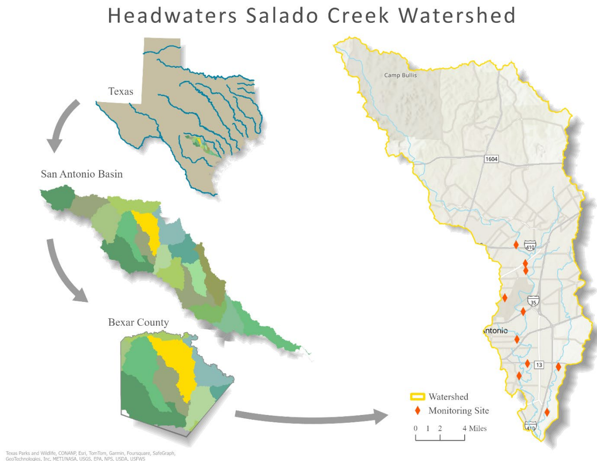
Figure 1. Salado Creek watershed in Bexar County, Texas
