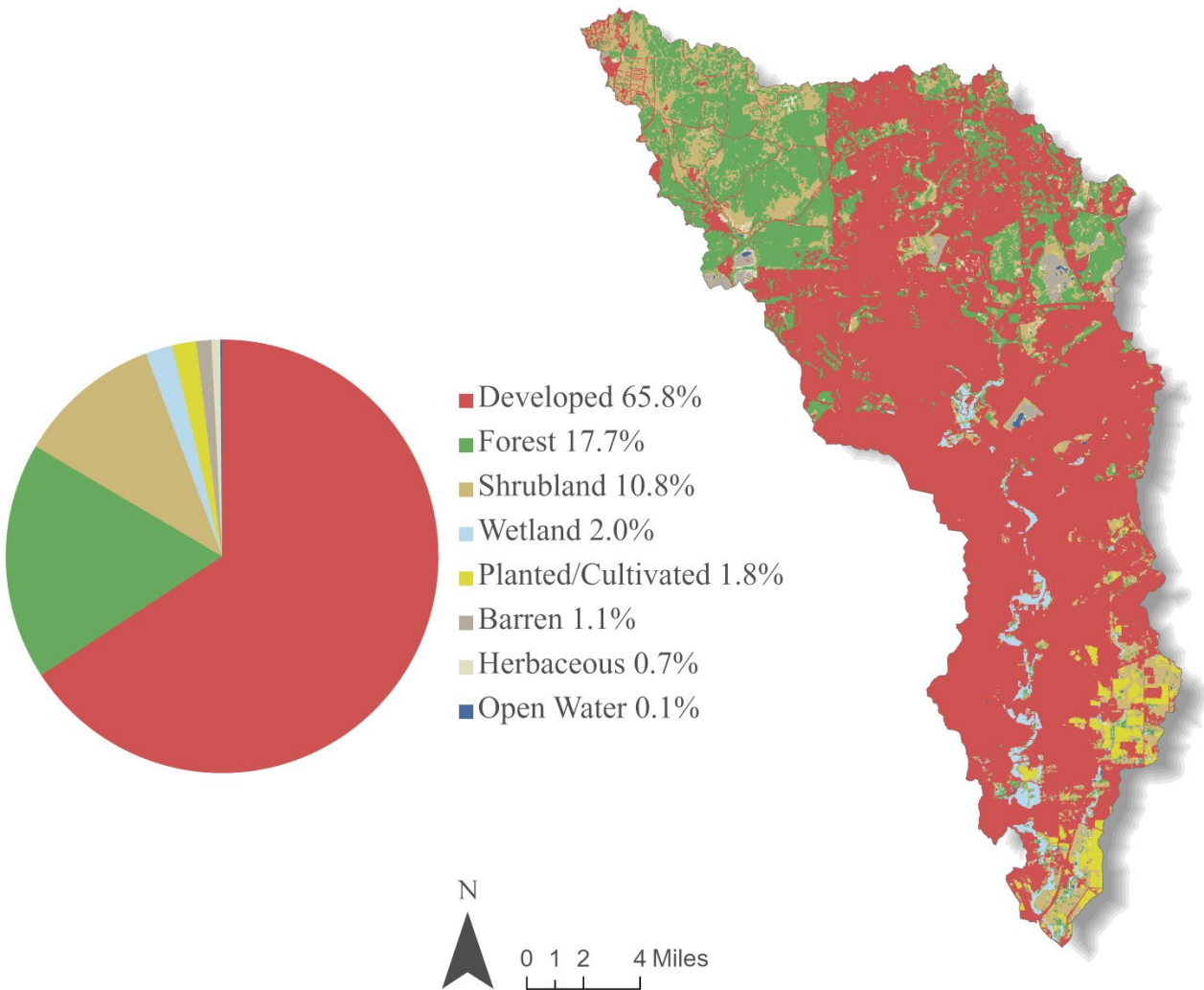
Figure 3. 2019 land use and land cover for the Salado Creek watershed in Bexar County, Texas (National Land Cover Data, 2019).
