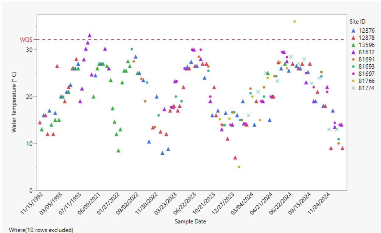
Figure 6. Water Temperature for Texas Stream Team sites in the Headwaters of Salado Creek watershed in Bexar County, Texas (November 1992 to January 2025). WQS = Water Quality Standard.
