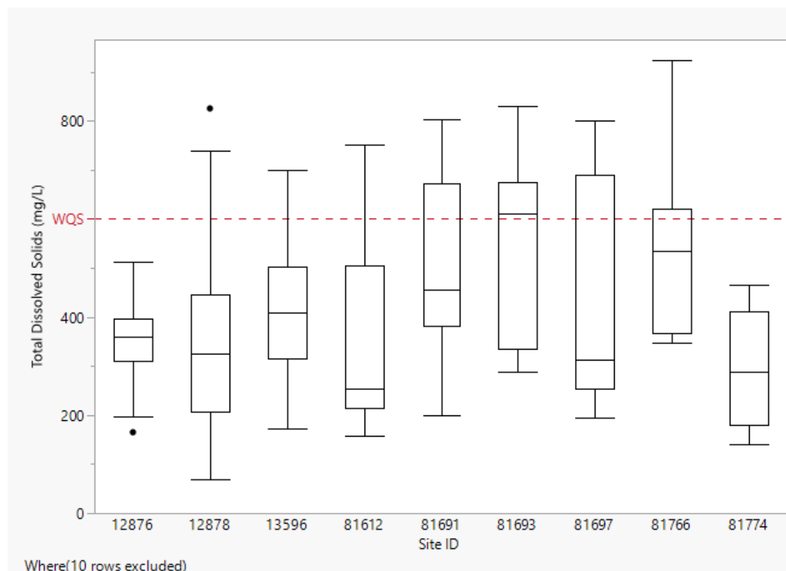
Figure 7. Total Dissolved Solids for Texas Stream Team sites in the Headwaters of Salado Creek watershed in Bexar County, Texas (November 1992 to January 2025). WQS = Water Quality Standard.
