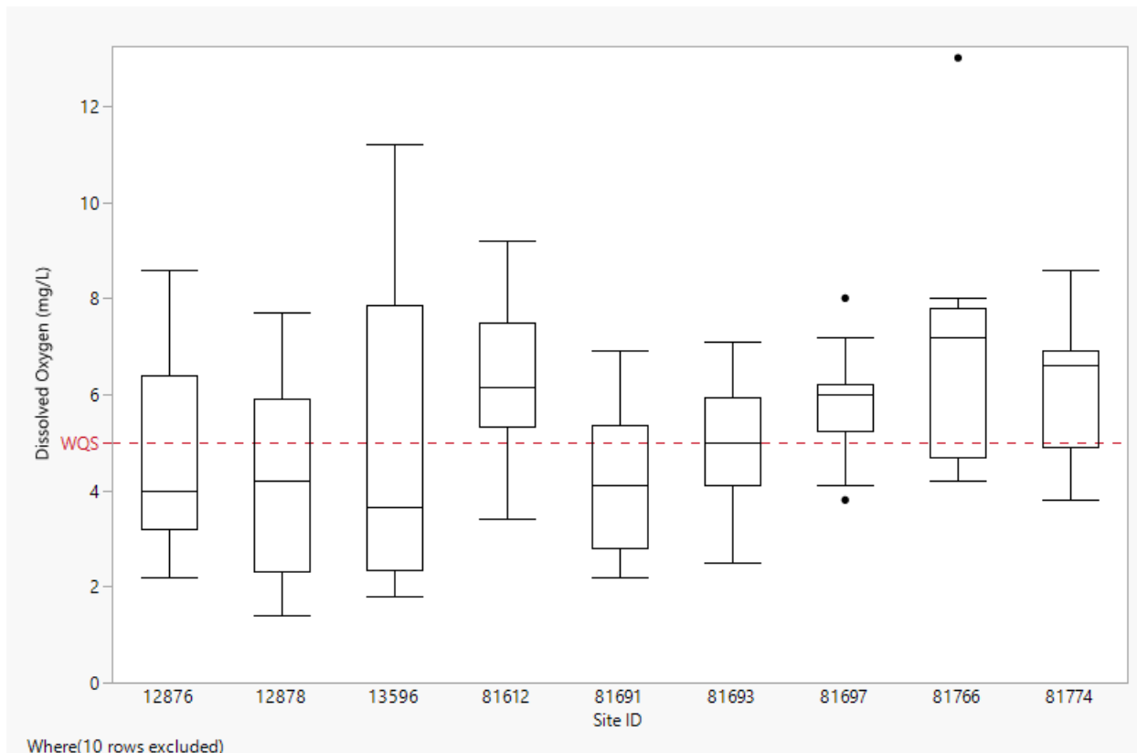
Figure 8. Dissolved Oxygen for Texas Stream Team sites in the Headwaters of Salado Creek watershed in Bexar County, Texas (November 1992 to January 2025). WQS = Water Quality Standard.
