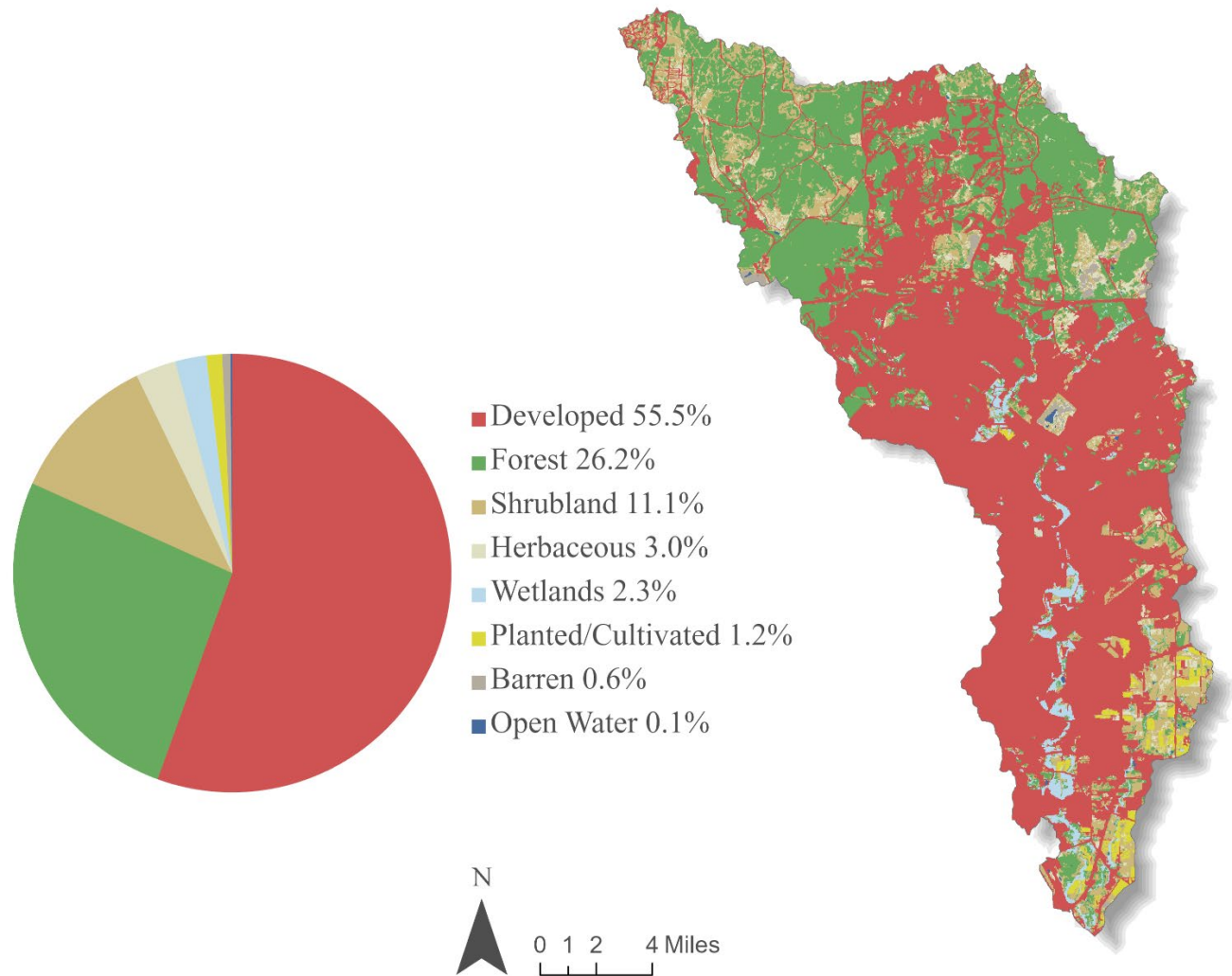
Figure 4. 2001 land use and land cover for the Salado Creek watershed in Bexar County, Texas (National Land Cover Data, 2001).
