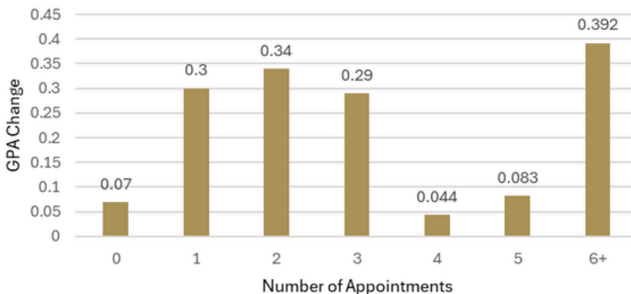
Average Semester to Semester GPA Change - 2024-2025 Year
