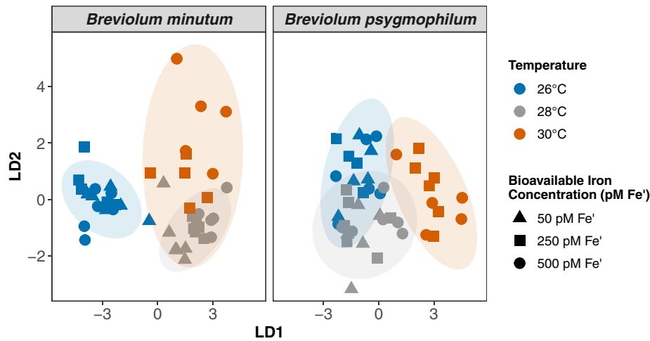
FIG. 3. A Discriminant function analysis (DFA) of metal concentrations ( \text{pg metal} \cdot \text{cell}^{-1} ) exhibits how clustering patterns distinctive to (A) Breviolum minutum and (B) B. psysgmophilum are correspond to different temperature thresholds. Alterations of B. minutum metal contents reflected heat stress at 28 and 30°C. In contrast, significant shifts of B. psysgmophilum in metal content did not occur until temperatures reached 30°C. The temperature thresholds associated with the two species were reflected in the success of their classification rates. High levels of misclassification occurred for B. psysgmophilum samples exposed to lower temperatures (68.8% correctly classified at 26°C, 64.7% at 28°C) whereas 91% of samples exposed to the highest temperature (30°C) were correctly classified. Contrastingly, 94% of B. minutum samples exposed to the lowest temperature (26°C) were correctly classified whereas misclassification of conspecifics exposed to higher temperatures was more frequent (88.2% correctly classified at 28°C, 60% at 30°C).
