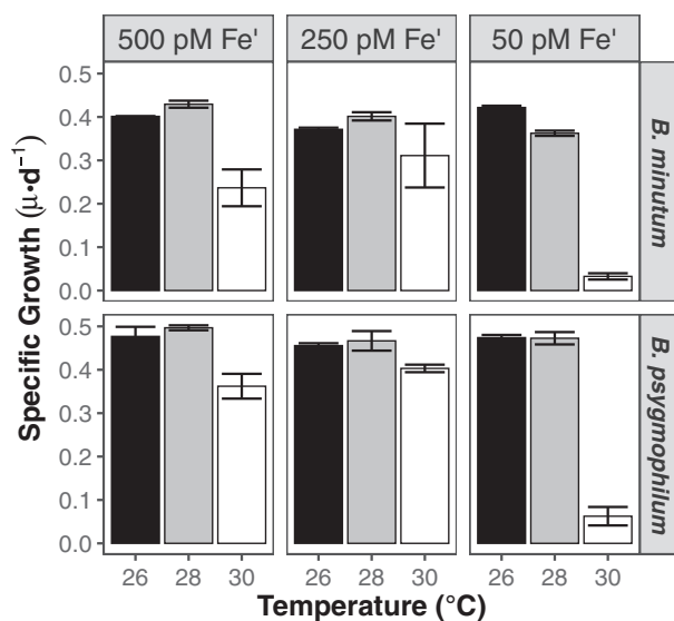
FIG. 1. Specific growth rate ( \mu \cdot \text{d}^{-1} ) of Breviolum spp. grown in different iron concentrations and temperatures. At higher iron concentrations, each species can withstand high temperatures, but cannot survive at 30°C when grown with low iron concentrations (50 pM Fe'). Breviolum psygmophilum grew 12–52% faster than B. minutum at all conditions. Bars represent the average of n = 3 replicates per treatment. Error bars represent \pm standard deviation.
