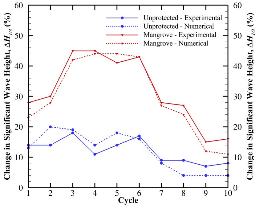
Figure 18. Change in significant wave height ( \Delta H_{1/3} ) between WG5 and WG6 for unprotected and mangrove-protected configurations.
