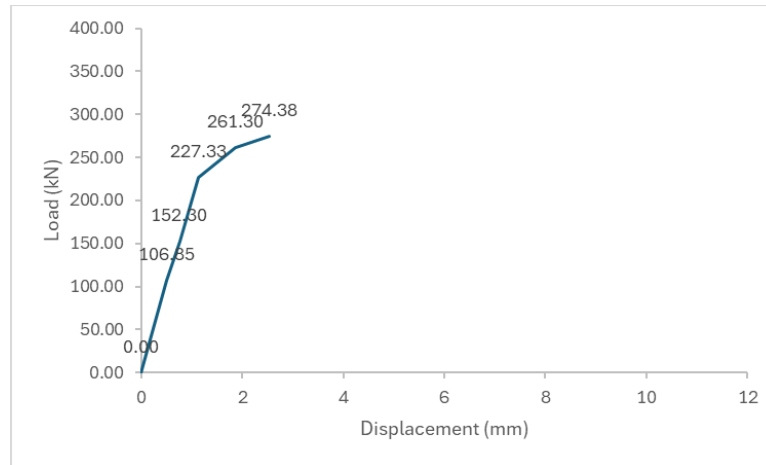
Figure 44: Load-displacement curve of specimen D1
