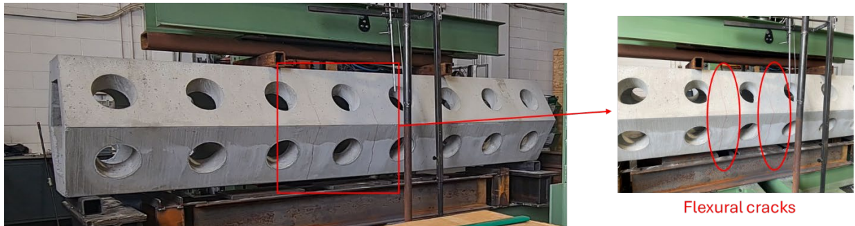
Figure 32: Flexural crack formation at specimen C1
