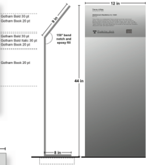
3 Exterior Plaque Pedestal
