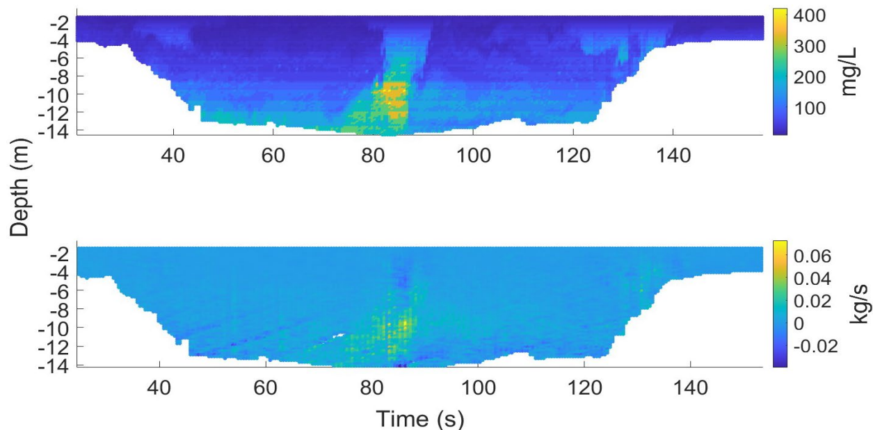
Figure 33. Comparison of SSC (top) and flux (bottom) produced by simultaneous passage of tugs BUD SONIER (top right of channel), MICHELLE ELISE (top left of channel), and deep-draft vessel BRENT HOLMEN (channel center).
