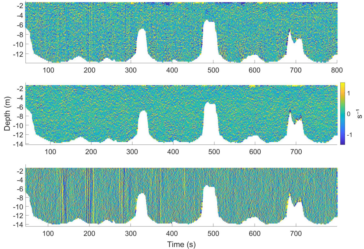
Figure 30. Measured x-vorticity (top), y-vorticity (center), z-vorticity (bottom) produced by vessel DESPINA V highlighting dipole vortices. Positive (yellow) vorticity indicates counterclockwise rotation, while negative (dark blue) vorticity indicates clockwise rotation.
