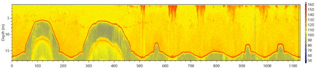
Figure 3. Raw vessel-mounted echosounder data from Corpus Christi Bay, Texas (Figlus and Song, 2020), analyzed for suspended sediment concentration by Gadgil (2021).
