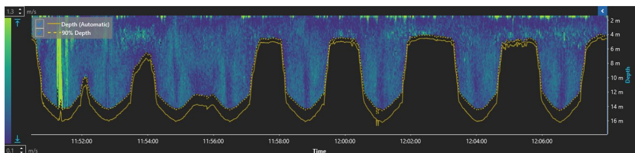
Figure 18. Example current profile time series from Signature VM Review application.
