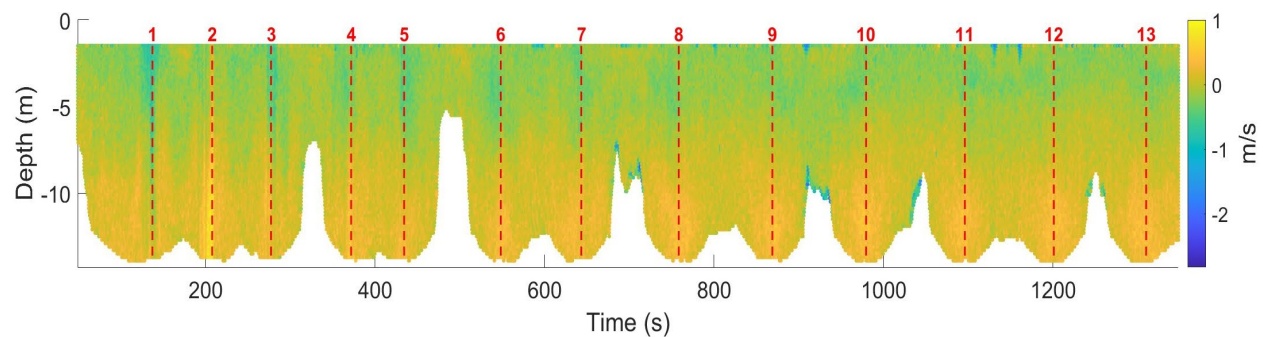
Figure 24. Measured velocity parallel with the channel produced by vessel UOG DESPINA V. Positive velocities (yellow) indicate flow moving away from the vessel negative velocities (blue) are moving towards the vessel.
