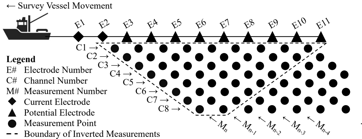
Figure 23. Apparent electrical resistivity pseudo-section, not to scale. Towed electrode cable shown behind survey vessel, moving left. E1 and E2 are current transmission electrodes, the remaining electrodes are used for voltage potential. The collected measurements are shown by solid circles with channel number increasing with depth and measurement number increasing to the left. Data outside the boundary of inverted measurements are not used for post-processing.
