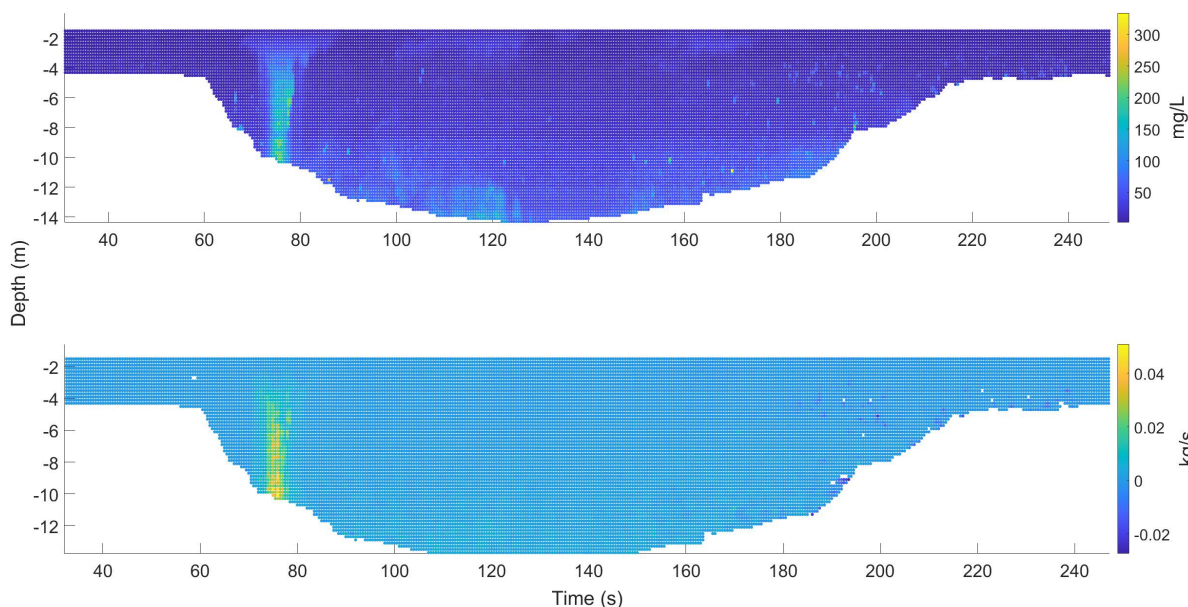
Figure 34. SSC (top) and suspended sediment flux (bottom) generated by vessel GOOD SHEPHERD. Positive (yellow) flux indicates sediment moving away from the vessel, while negative (blue) flux indicates sediment moving towards the vessel.
